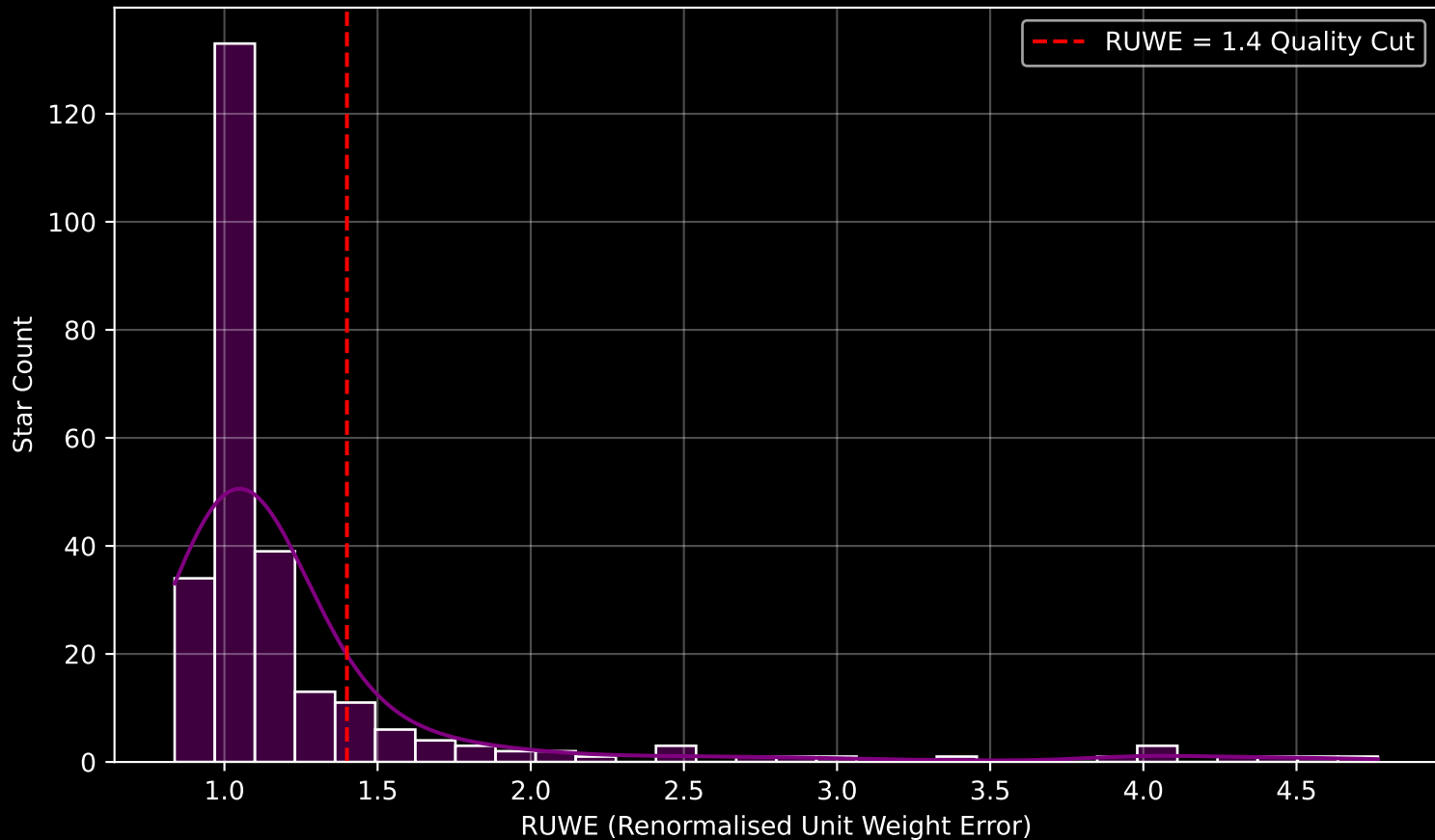
GALAH DR4 Field [2176] RUWE Distribution (n= 263)
