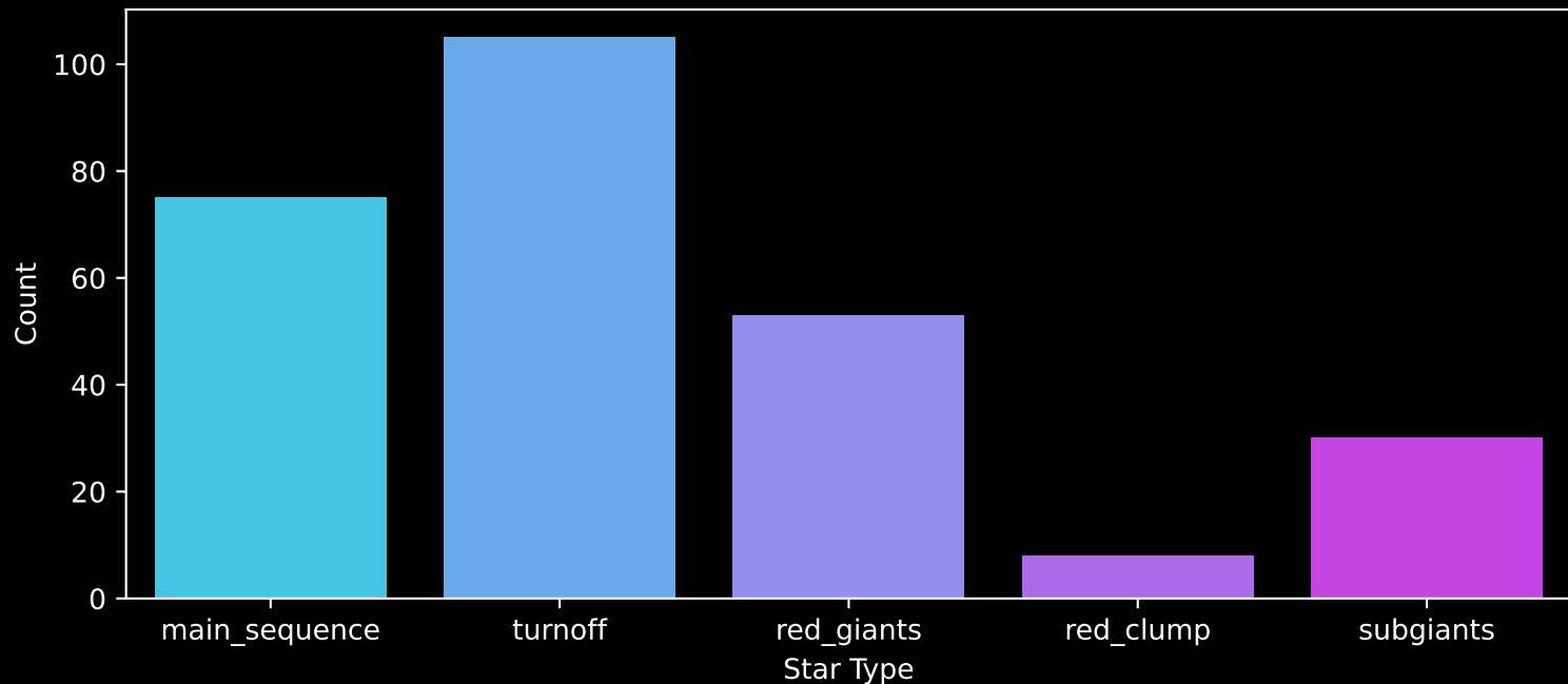
GALAH DR4 Field: [2176] Count plot of Star Type
