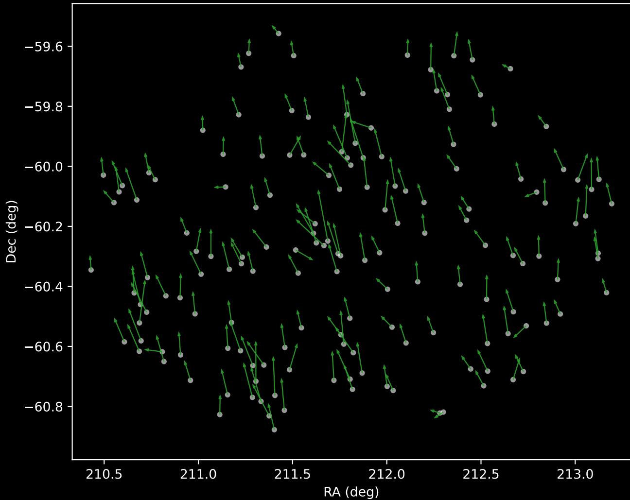
GALAH DR4 Cluster 4 Proper Motion Vectors (n=157)
